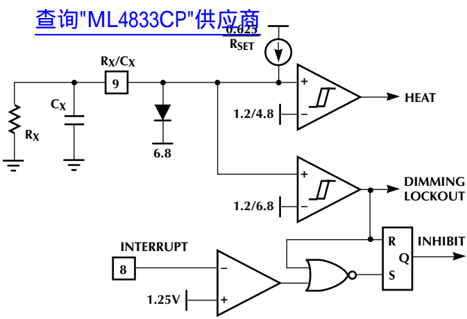
Figure 8. Lamp Preheat and Interrupt Timers LFB OUT is ignored by the oscillator until C_X reaches 6.8V threshold. The lamps are therefore driven to full power and then dimmed. The C_X pin is clamped to about 7.5V.
