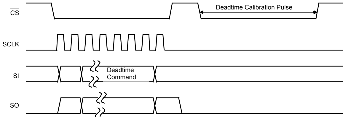
Figure 21. Deadtime Calibration
