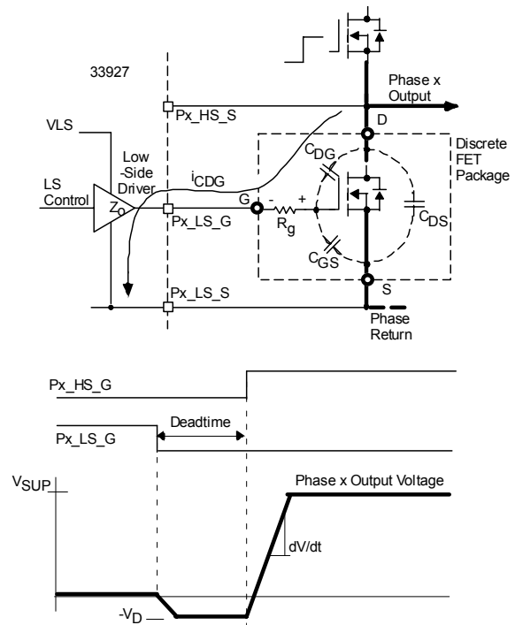
Figure 17. Positive DV/dt Transient
