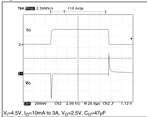
Figure 17. Load transient
