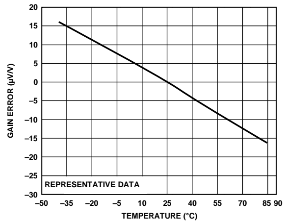
Figure 11. Gain Error vs. Temperature, Normalized at 25 ^\circ\text{C}
