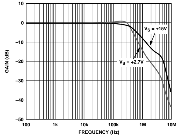
Figure 12. Gain vs. Frequency, V_S = \pm 15\text{ V} , +2.7 V
