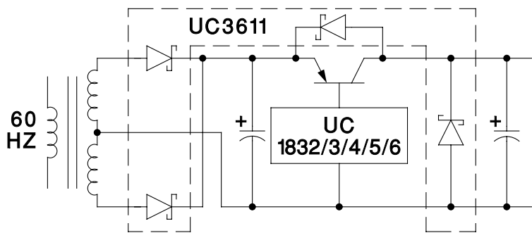
Figure 5. Linear Regulations
