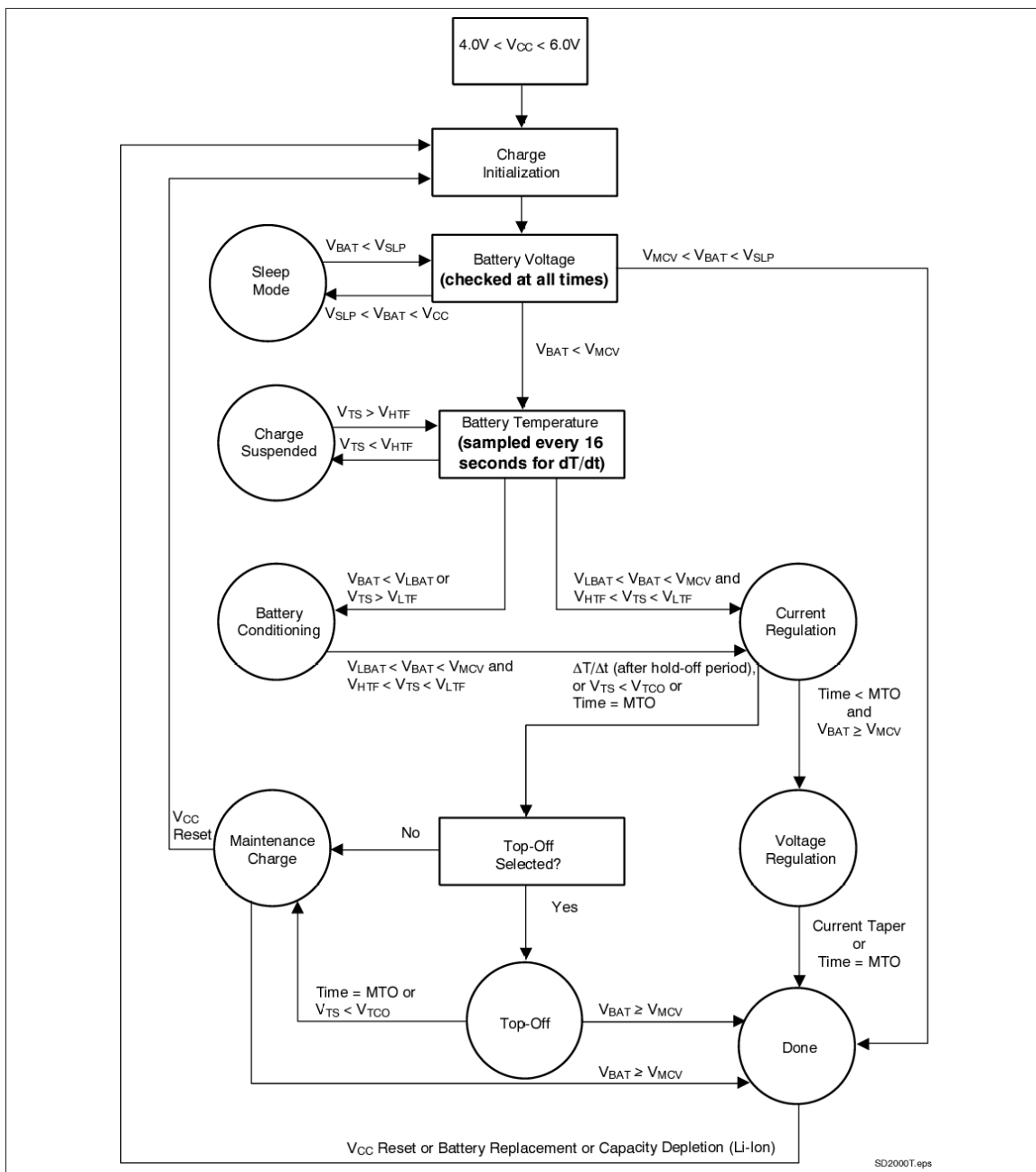
Figure 2. State Diagram
