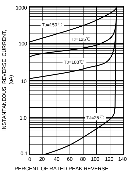
FIG.5-TYPICAL REVERSE CHARACTERISTICS
