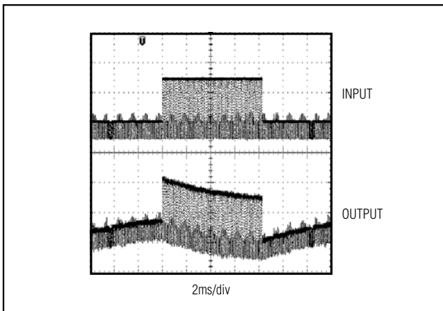
Figure 1. AC-Coupled Output
