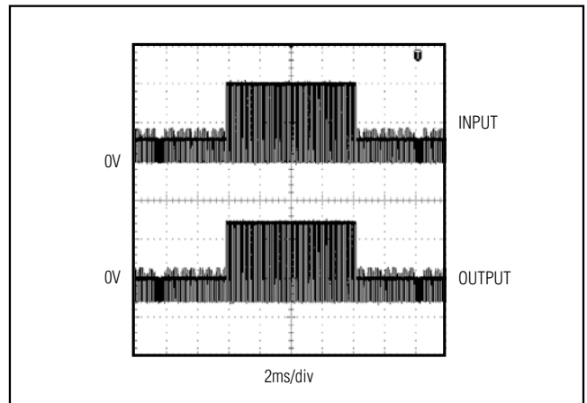
Figure 2. DirectDrive Output
