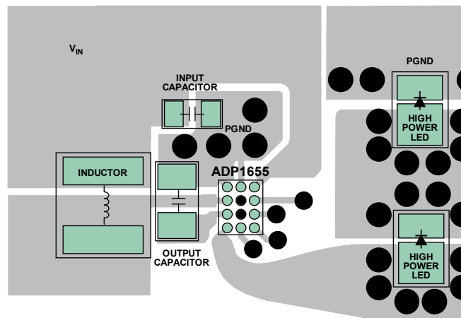
Figure 36. Example Layout of the ADP1655 Driving Two White LEDs
