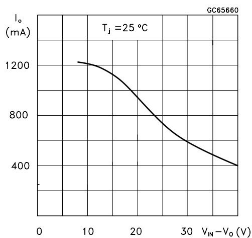
Figure 4: Current Limit
