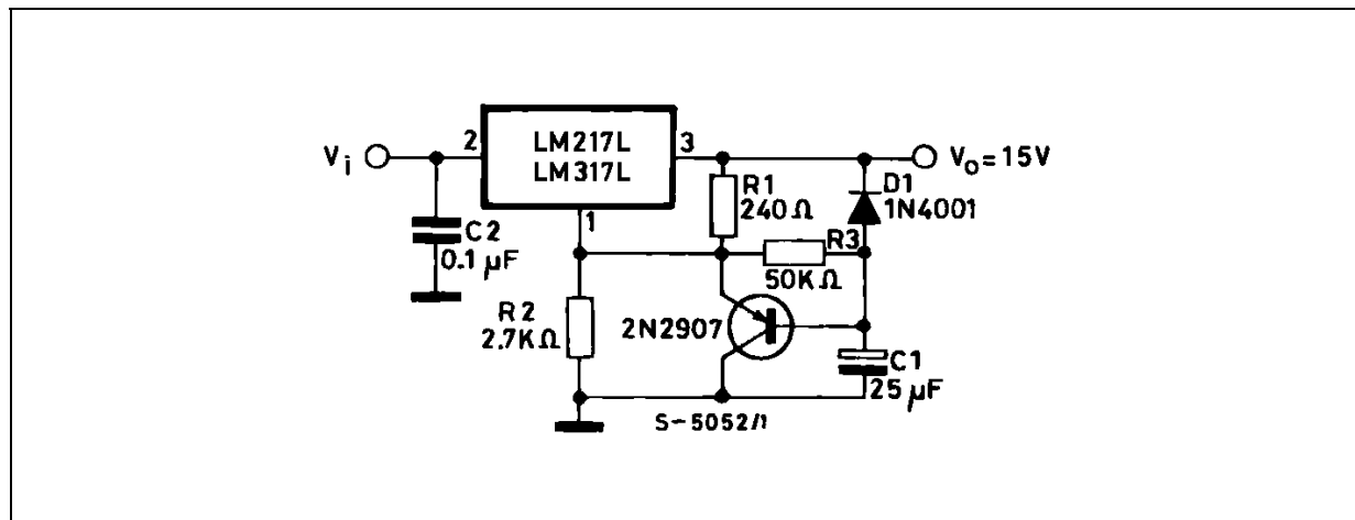
Figure 9: Current Regulator
