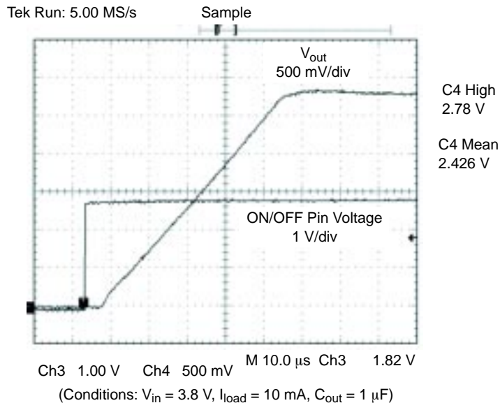
Figure 12. Start-Up Waveform
