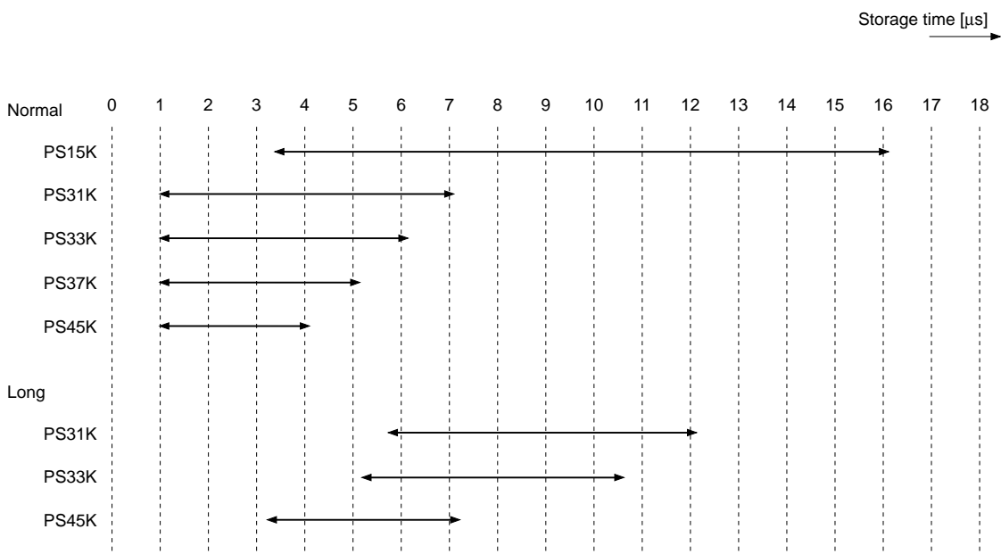
Fig. 2. Reference Example of Supported Storage Times for Each Mode (H-pulse Width: 4.5μs)
