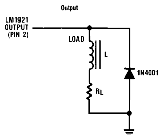
FIGURE 2. Diode Clamp
