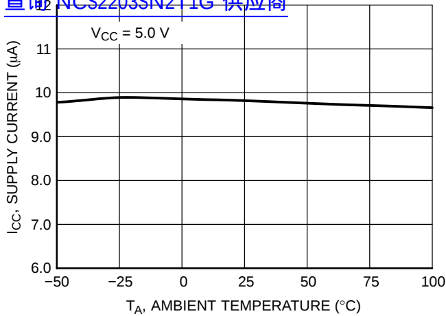
Figure 1. NCS2200 Series Supply Current versus Temperature
