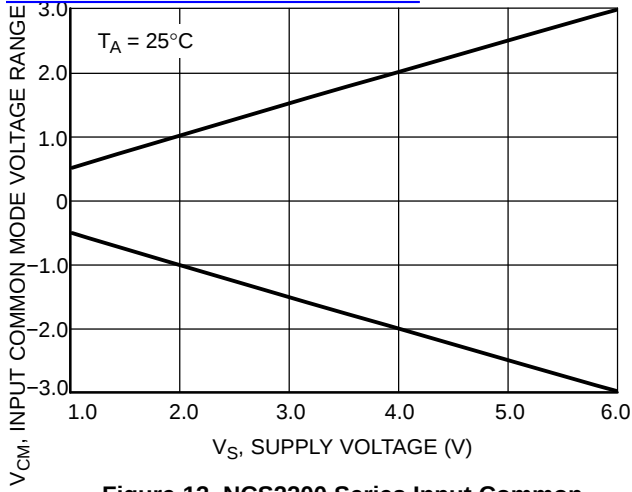
Figure 13. NCS2200 Series Input Common Mode Voltage Range versus Supply Voltage
