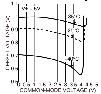
Offset Voltage vs. Common-Mode Voltage
