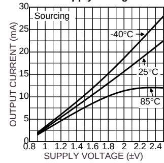
Short Circuit Current vs. Supply Voltage
