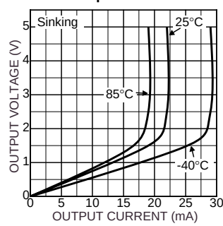
Output Voltage vs. Output Current
