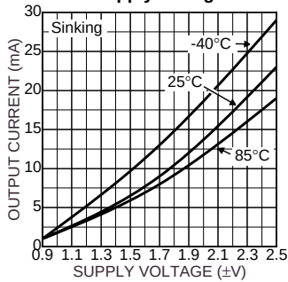
Short Circuit Current vs. Supply Voltage
