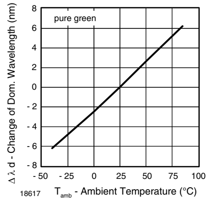
Figure 7. Change of Dominant Wavelength vs. Ambient Temperature
