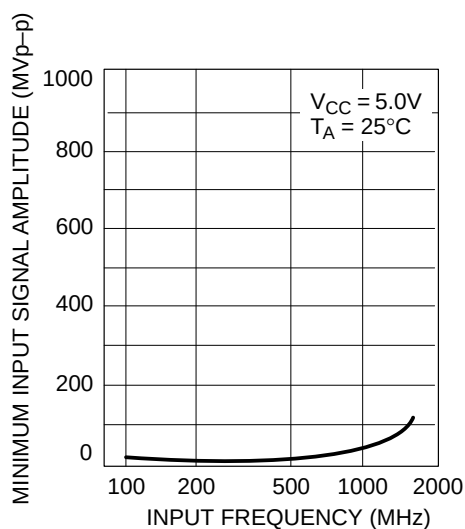
Figure 2. Input Signal Amplitude vs. Input Frequency
