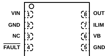
ISL9211 (8 LD 2x2 \mu TDFN) TOP VIEW
