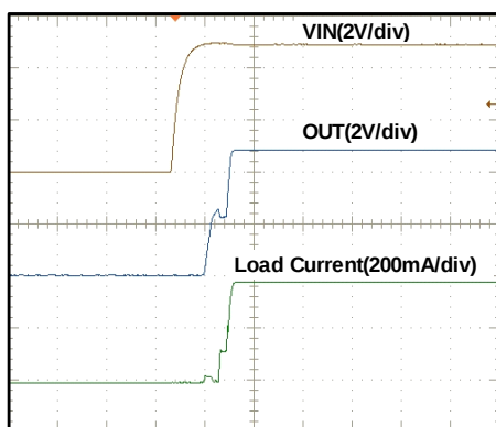
FIGURE 2. CAPTURED WAVEFORMS FOR POWER-UP. THE OUTPUT IS LOADED WITH A 10Ω RESISTOR
