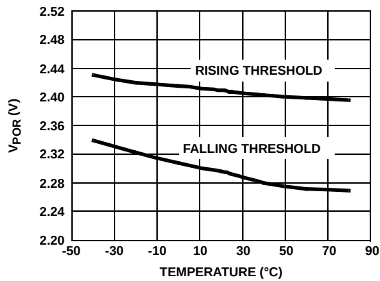
FIGURE 10. V_{POR} vs TEMPERATURE
