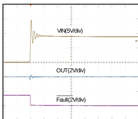
FIGURE 6. TRANSIENT WAVEFORMS WHEN INPUT STEPS FROM ZERO TO 9V
