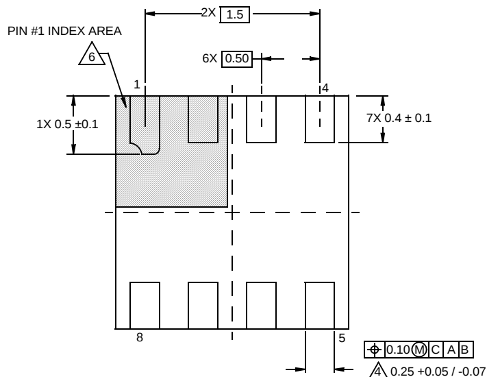
BOTTOM VIEW
