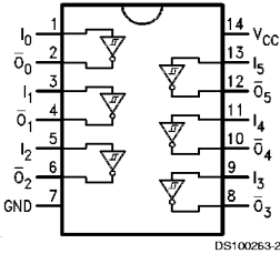
Pin Assignment for DIP and Flatpack
