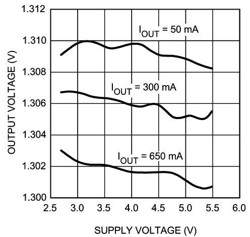
Output Voltage vs Supply Voltage ( V_{OUT} = 1.3V )
