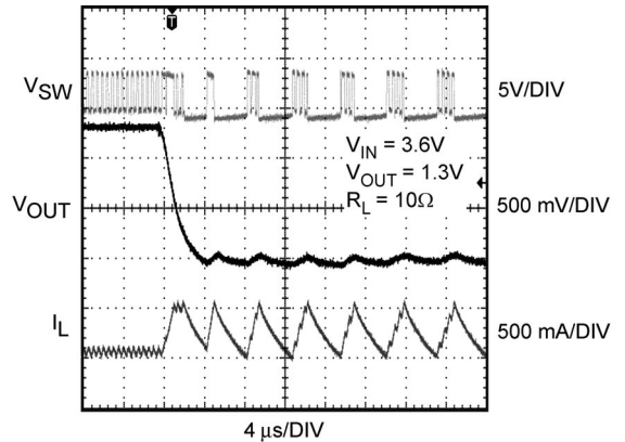
Timed Current Limit Response ( V_{IN} = 3.6V )
