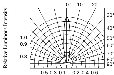
FIG.6 RADIATION DIAGRAM
