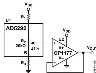
Figure 51. Optimizing Resolution
