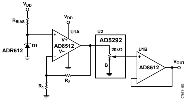
Figure 49. High Voltage DAC
