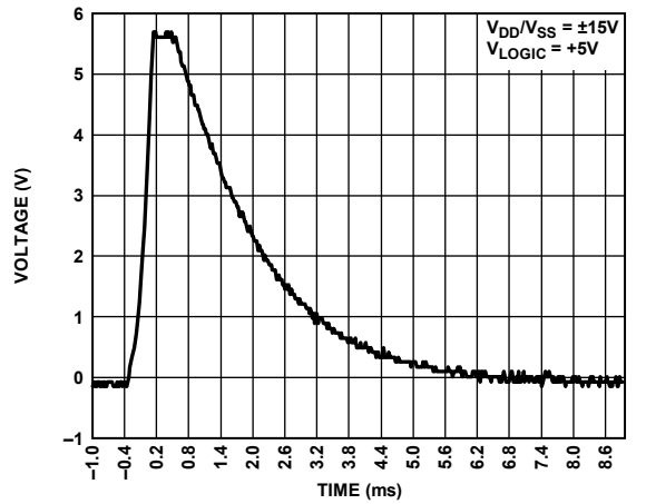
Figure 34. V_{EXT\_CAP} Waveform While Reading Fuse or Calibration
