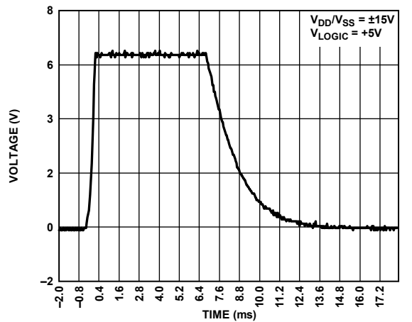
Figure 35. V_{EXT\_CAP} Waveform While Writing Fuse
