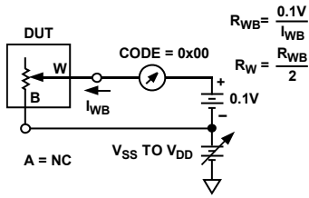
Figure 39. Wiper Resistance
