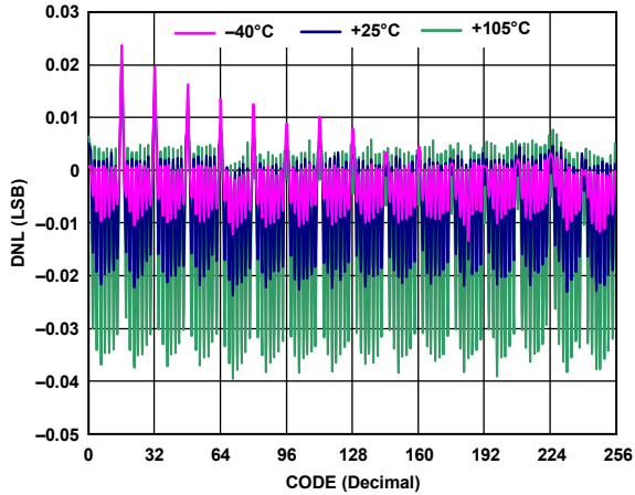
Figure 13. R-DNL in Normal Mode vs. Code vs. Temperature (AD5291)
