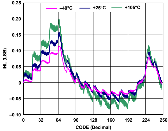
Figure 12. R-INL in Normal Mode vs. Code vs. Temperature (AD5291)
