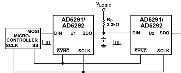
Figure 43. Daisy-Chain Configuration Using SDO
