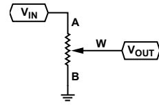
Figure 46. Potentiometer Mode Configuration
