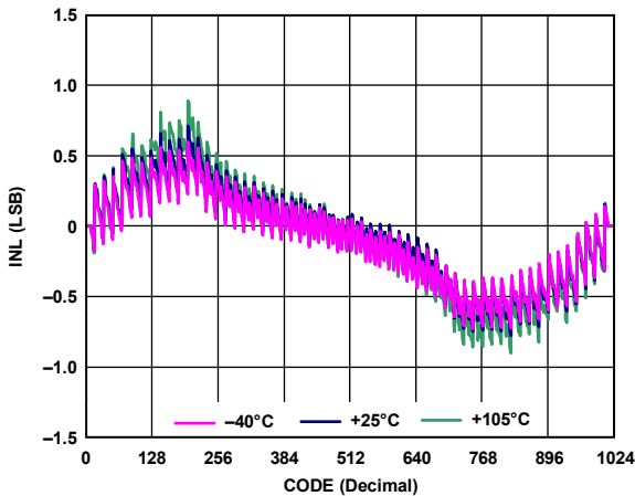
Figure 14. INL in R-Perf Mode vs. Code vs. Temperature (AD5292)
