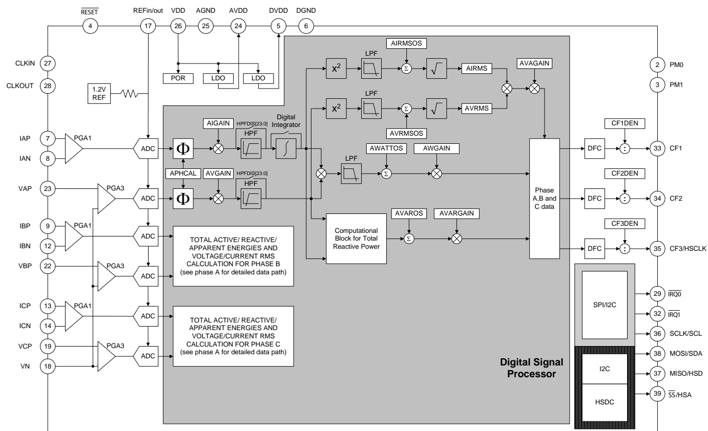
Figure 1. ADE7858 Functional Block Diagram
