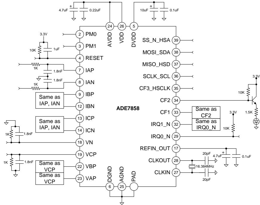
Figure 7. Test Circuit
