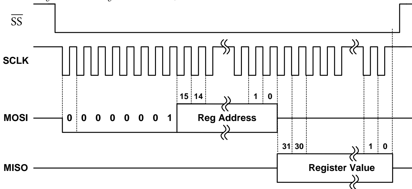
Figure 63. SPI read operation of a 32-bit register
