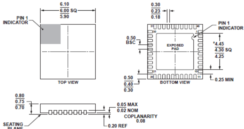
Figure 69. 40-Lead Lead Frame Chip Scale package [LFCSP_WQ], 6 x 6 mm Body, Very Very Thin Quad (CP-40-10) Dimensions shown in millimeters
