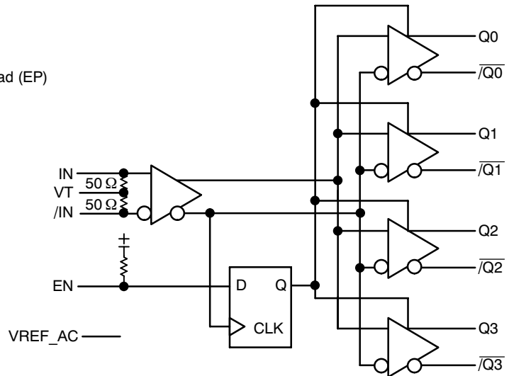
Figure 3. Logic Diagram
