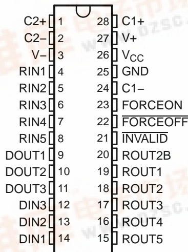
DB OR PW PACKAGE (TOP VIEW)
