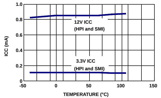
FIGURE 21. ICC CURRENT vs TEMPERATURE
