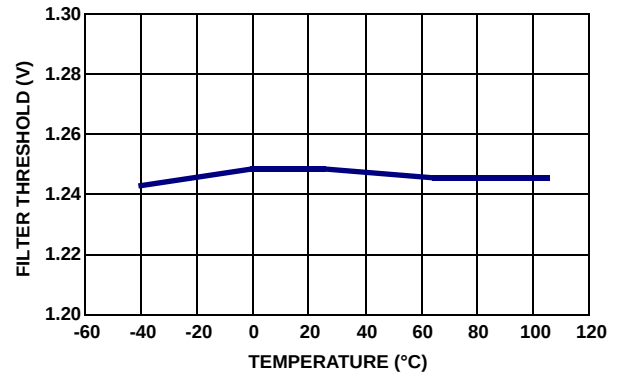
FIGURE 33. FILTER THRESHOLD VOLTAGE vs TEMPERATURE
