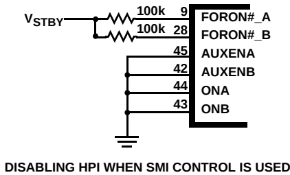
FIGURE 1. I/O CONFIGURATION FOR DISABLING HPI/SMI CONTROL
