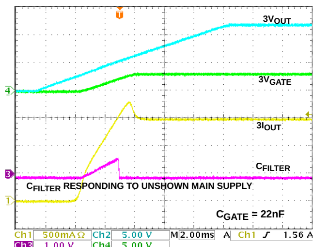
FIGURE 4. 3VMAIN START-UP R_{LOAD} = 2\Omega , C_{LOAD} = 470\mu F
