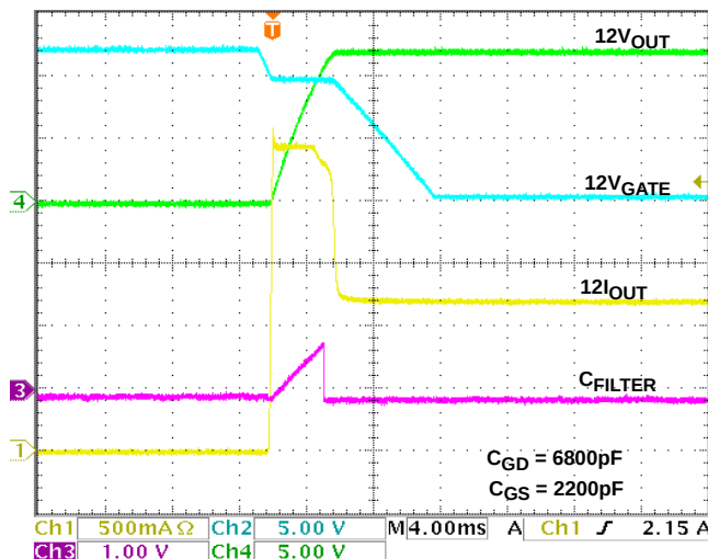
FIGURE 5. 12VMAIN START-UP R_{LOAD} = 10\Omega , C_{LOAD} = 470\mu F
