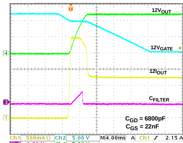
FIGURE 3. 12VMAIN START-UP R_{LOAD} = 10\Omega , C_{LOAD} = 470\mu F
