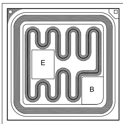
BACKSIDE COLLECTOR
