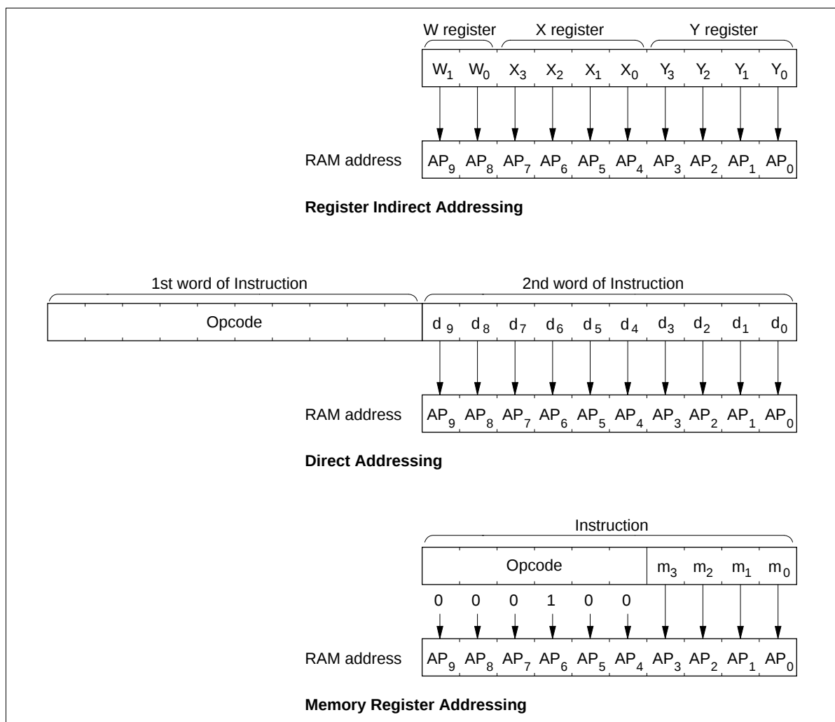
Figure 84 RAM Addressing Modes
