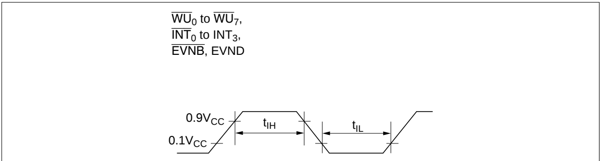
Figure 89 Interrupt Timing
