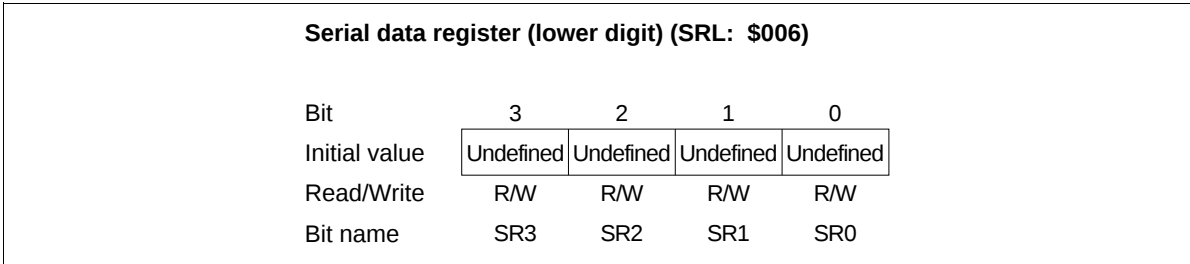
Figure 73 Serial Data Register Lower Digit (SRL)
