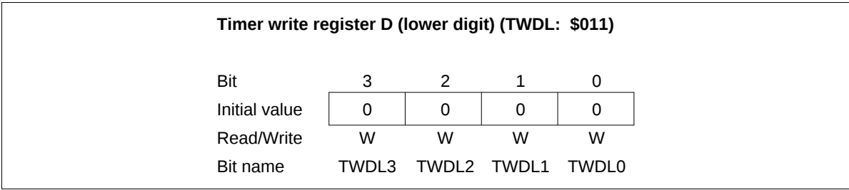
Figure 62 Timer Write Register D Lower Digit (TWDL)
