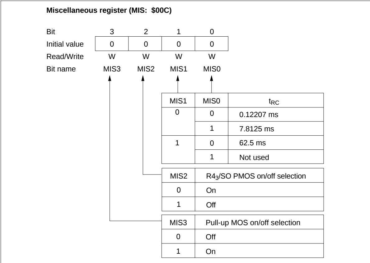
Figure 77 Miscellaneous Register (MIS)
