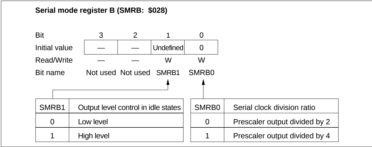
Figure 72 Serial Mode Register B (SMRB)
