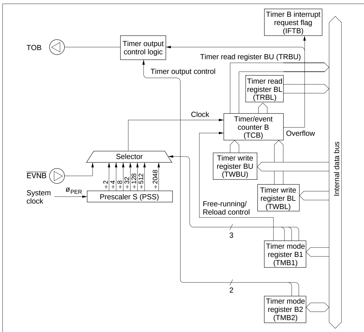
Figure 43 Block Diagram of Timer B
