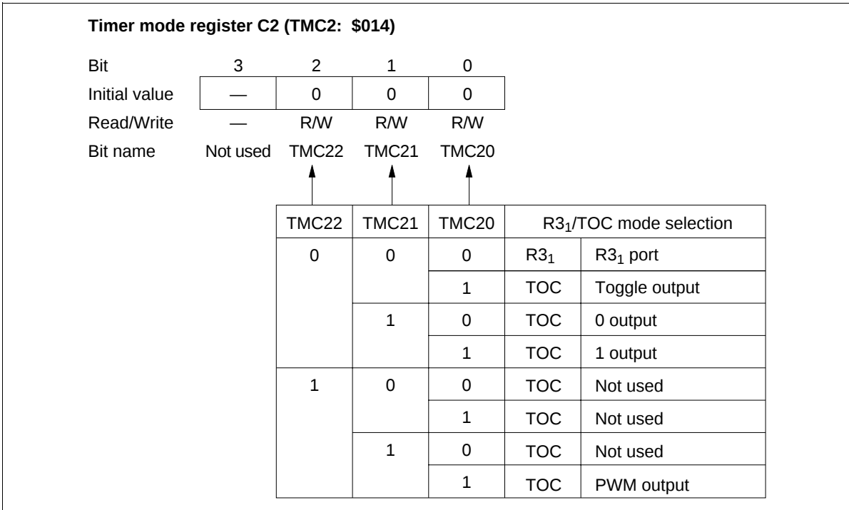
Figure 33 Timer Mode Register C2 (TMC2)
