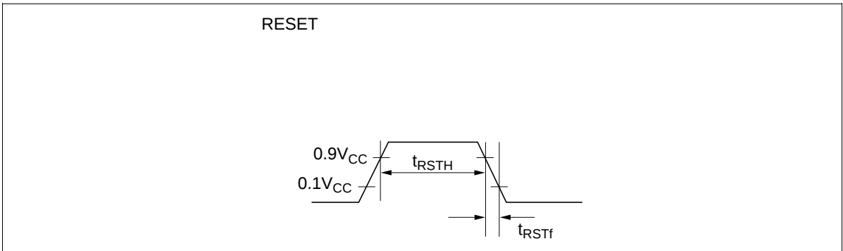
Figure 90 Reset Timing
