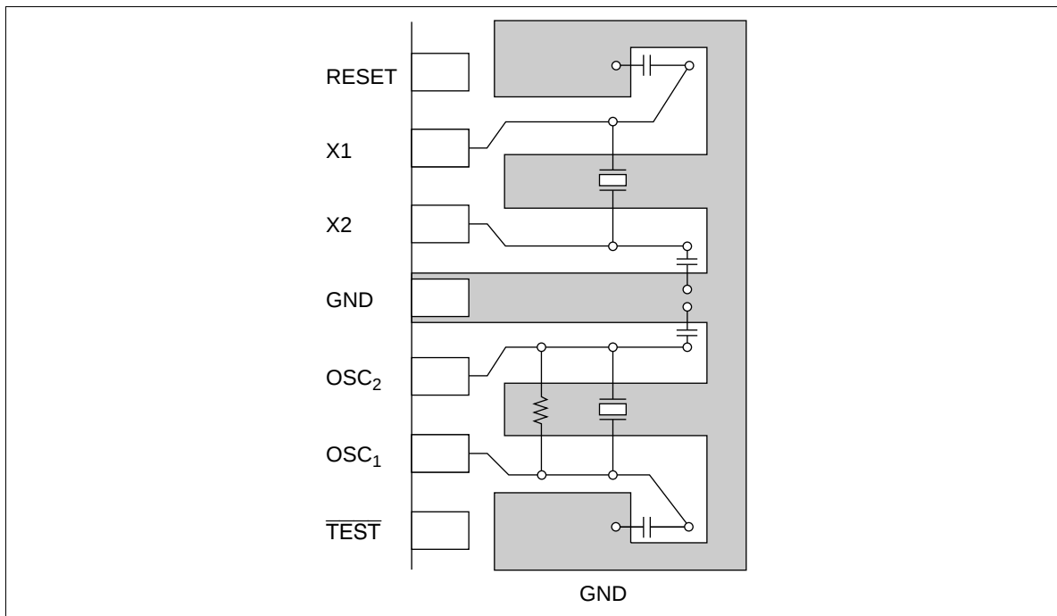
Figure 28 Typical Layout of Crystal and Ceramic Oscillators
