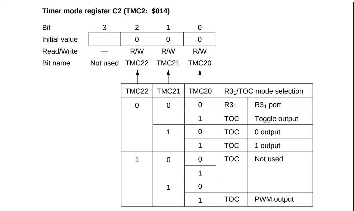
Figure 54 Timer Mode Register C2 (TMC2)
