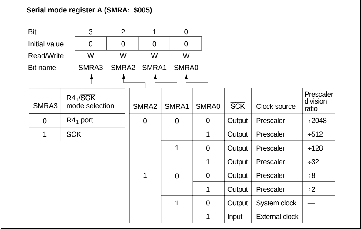
Figure 37 Serial Mode Register A (SMRA)
