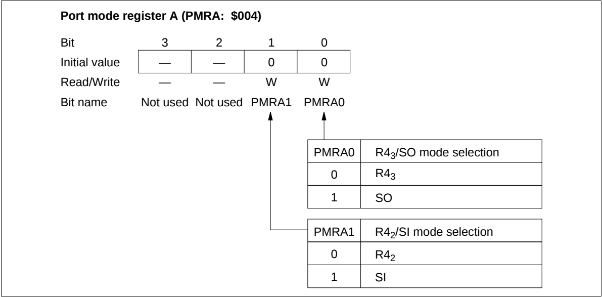
Figure 36 Port Mode Register A (PMRA)
