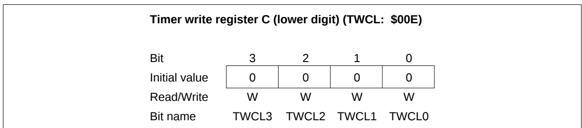
Figure 55 Timer Write Register C Lower Digit (TWCL)
