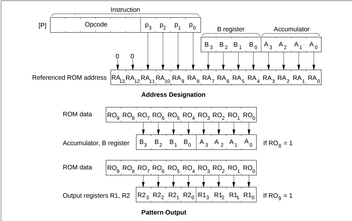
Figure 86 P Instruction
