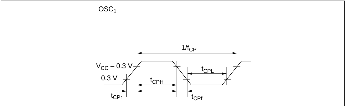
Figure 88 External Clock Timing
