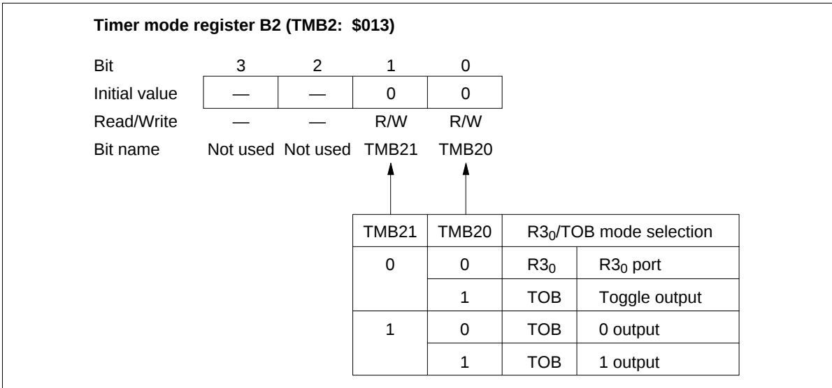
Figure 32 Timer Mode Register B2 (TMB2)
