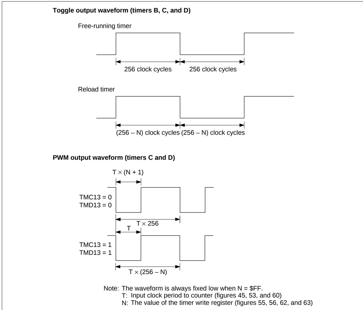
Figure 44 Timer Output Waveform
