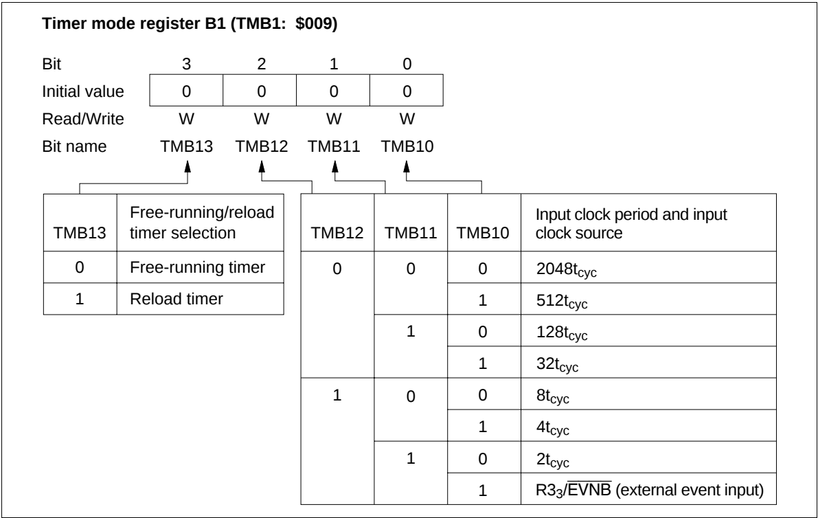
Figure 45 Timer Mode Register B1 (TMB1)
