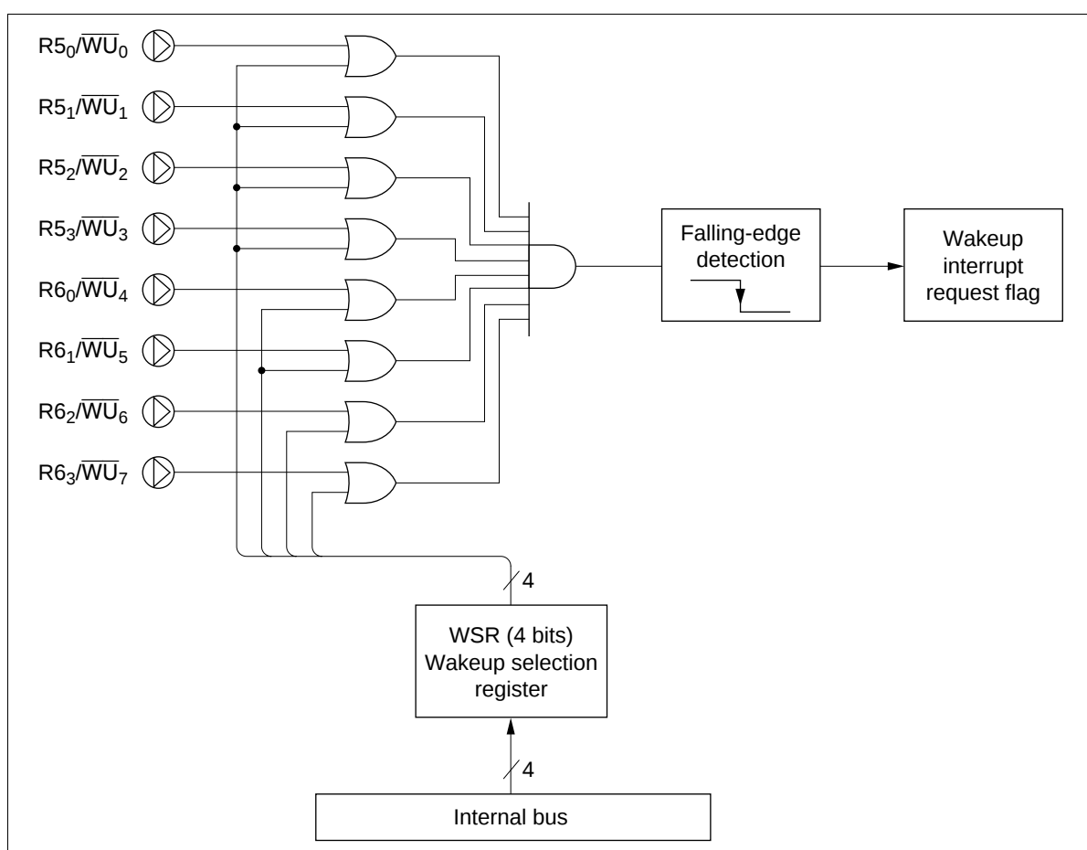
Figure 12 Wakeup Interrupt
