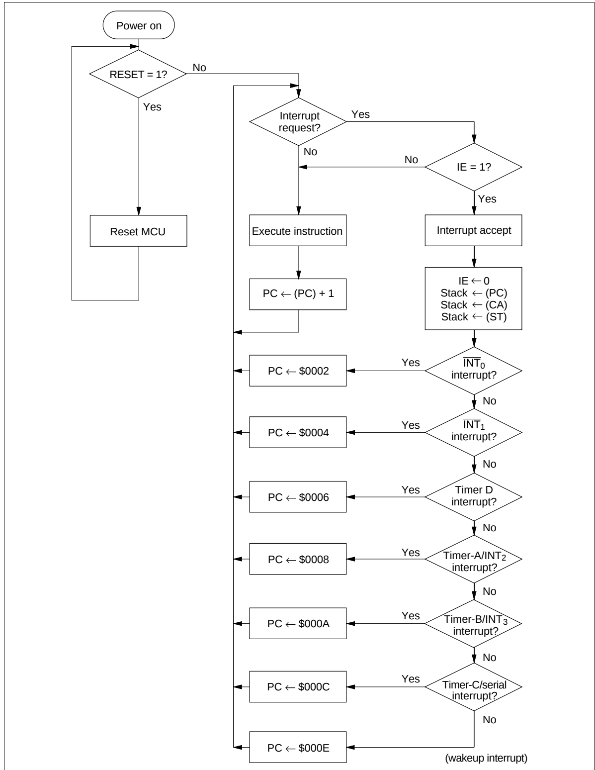
Figure 10 Interrupt Processing Flowchart
