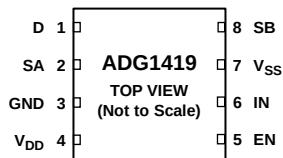
Figure 3. 8-Lead LFCSP Pin Configuration
