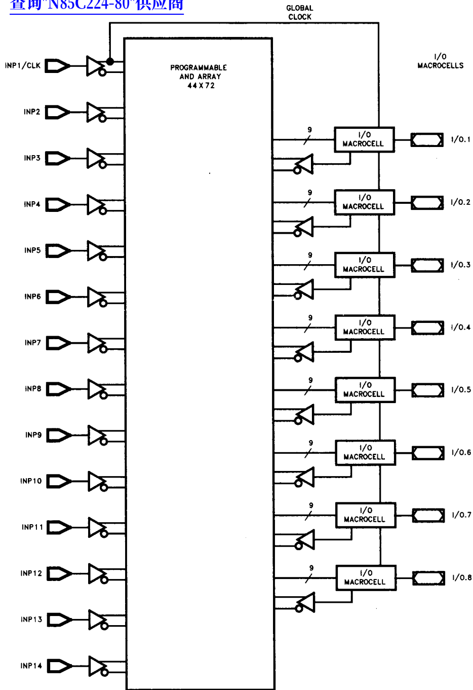
Figure 3. 85C224 Global Architecture
