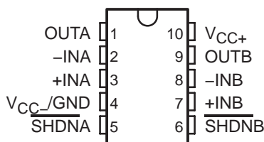
LMV982 . . . DGS (VSSOP/MSOP) PACKAGE (TOP VIEW)
