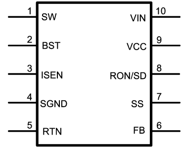
10-Lead LLP
