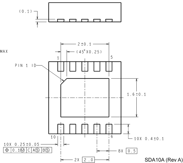
10-Lead LLP Package NS Package Number SDA10A
