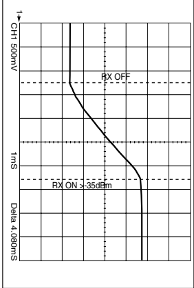
Figure 5: Worst Case RSSI Response Time
