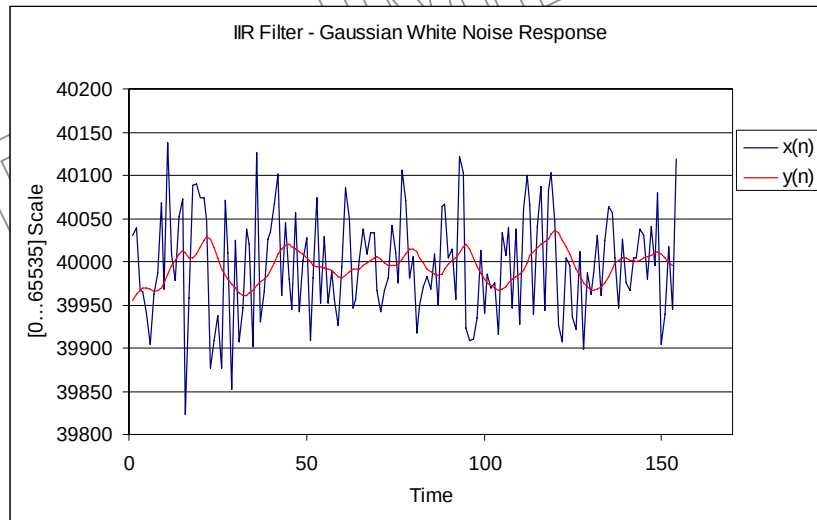
Figure 15 - Noise Response for the IIR Filter
