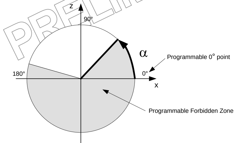
Figure 12 – Discontinuity Point and Dead Zone (Alpha – Idem ditto for Beta)
