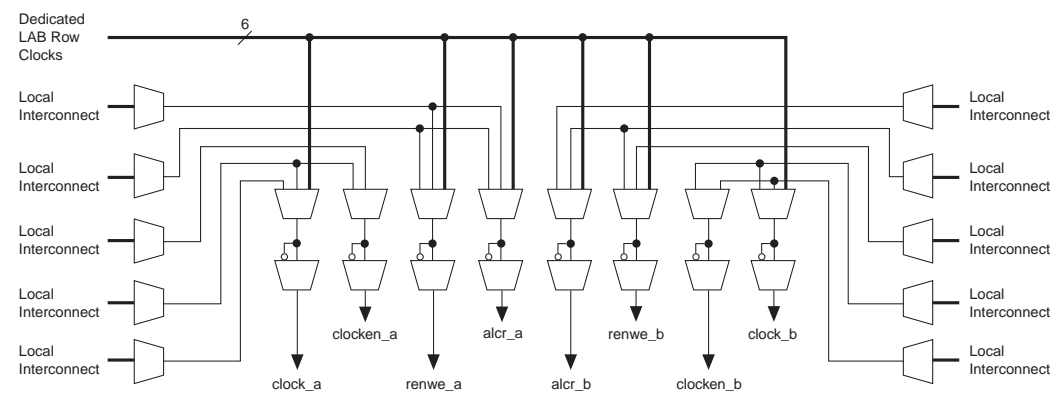
Figure 15. M4K RAM Block Control Signals
