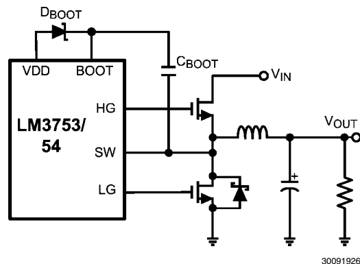
FIGURE 6. Bootstrap Circuit
