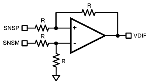
FIGURE 7. Differential Amplifier
