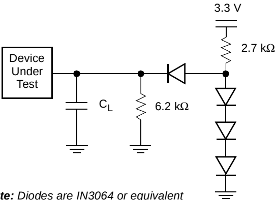
Figure 11. Test Setup
