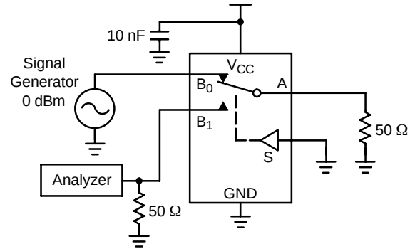
Figure 7. Crosstalk
