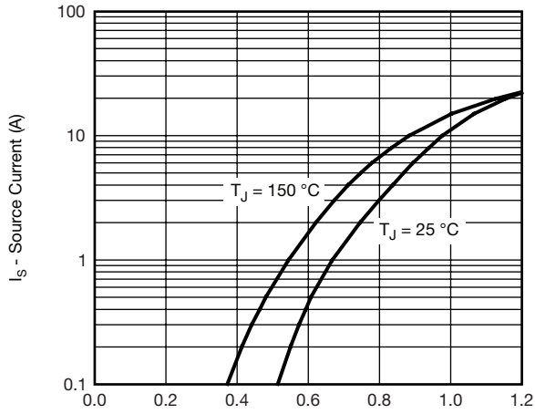
V_{SD} - Source-to-Drain Voltage (V) Soure-Drain Diode Forward Voltage
