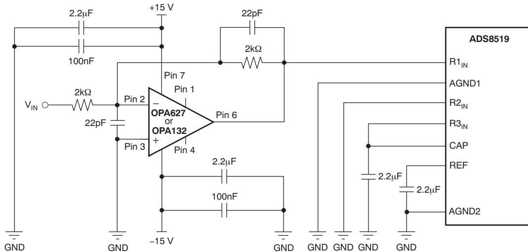
Figure 31. Typical Driving Circuitry ( \pm 10 V, No Trim)
