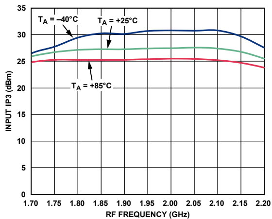
Figure 5. Input IP3 vs. RF Frequency
