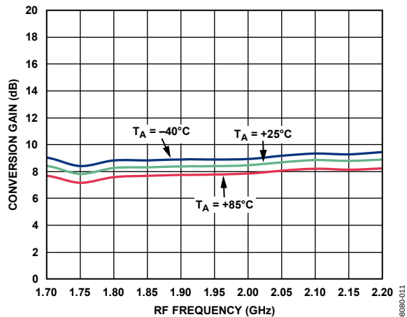
Figure 4. Power Conversion Gain vs. RF Frequency
