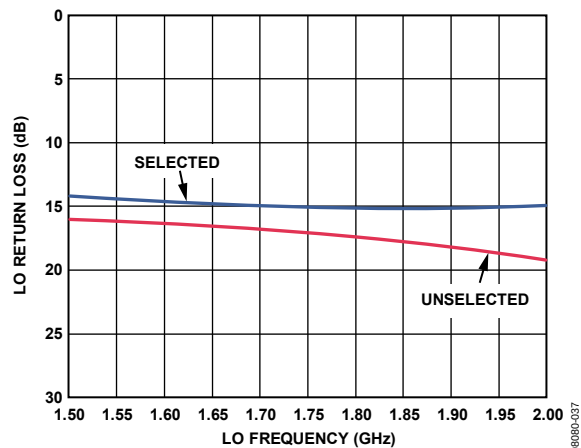
Figure 32. LO Return Loss, Selected and Unselected
