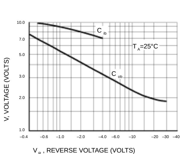
Figure 5. Capacitances
