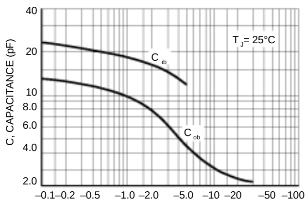
Figure 11. Capacitance
