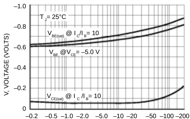
Figure 8. "On" Voltage
