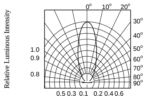
FIG.6 RADIATION DIAGRAM
