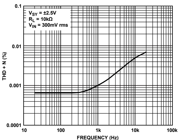
Figure 50. THD + Noise vs. Frequency
