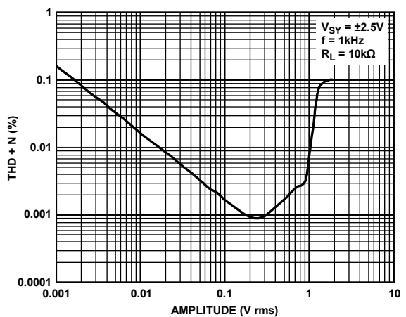
Figure 49. THD + Noise vs. Amplitude
