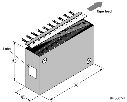
Figure 21. Tape Direction
