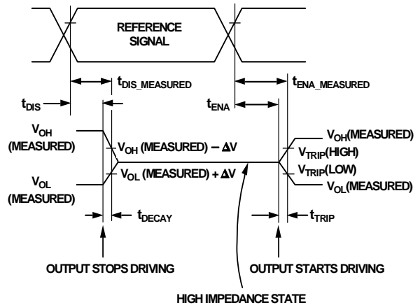
Figure 43. Output Enable/Disable
