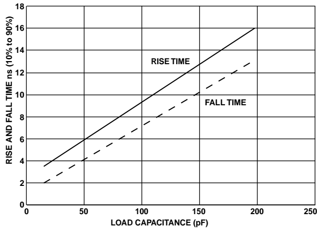
Figure 55. Typical Rise and Fall Times (10% to 90%) versus Load Capacitance for Driver D at V_{DDEXT} = 2.25\text{ V}
