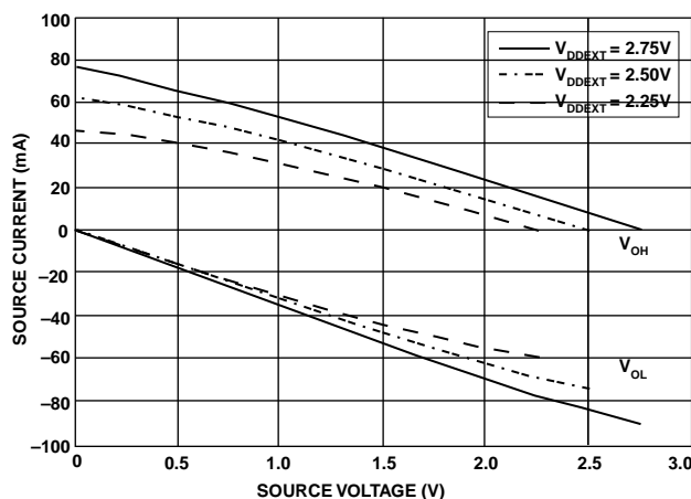
Figure 39. Drive Current D ( V_{DDEXT} = 2.5 \text{ V} )
