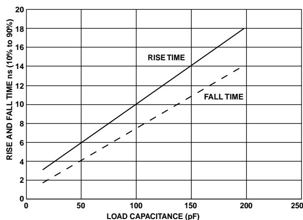
Figure 53. Typical Rise and Fall Times (10% to 90%) versus Load Capacitance for Driver C at V_{DDEXT} = 3.65\text{ V}
