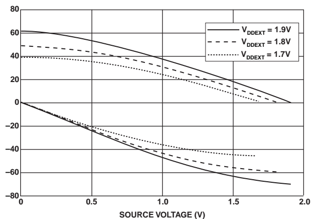
Figure 34. Drive Current B ( V_{DDEXT} = 1.8\text{ V} )
