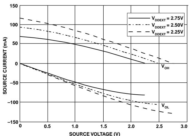
Figure 33. Drive Current B ( V_{DDEXT} = 2.5\text{ V} )
