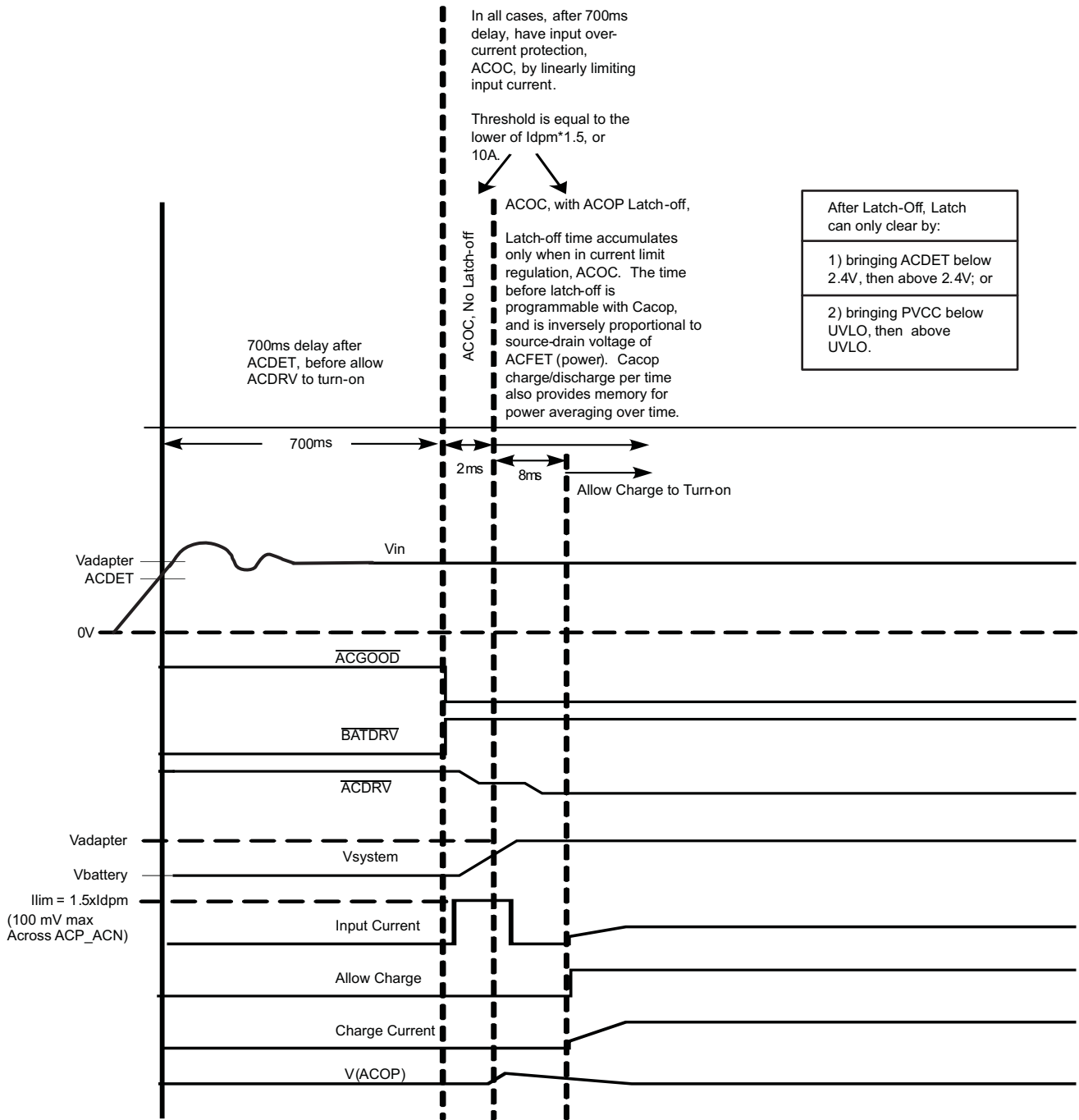
A. ACDET overpower protection; initial current limit allows safe soft-start without system voltage droop.
