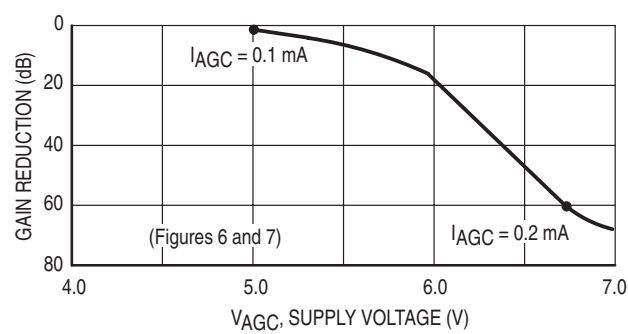
Figure 2. Typical Gain Reduction
