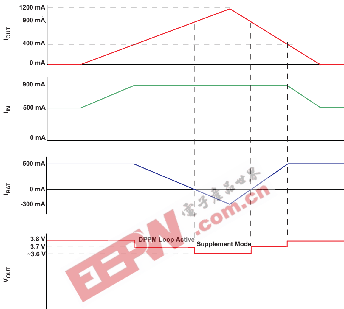
Figure 37. bq24072 DPM and Battery Supplement Modes ( V_{OREG} = V_{BAT} + 225\text{mV} , V_{BAT} = 3.6\text{V} )
