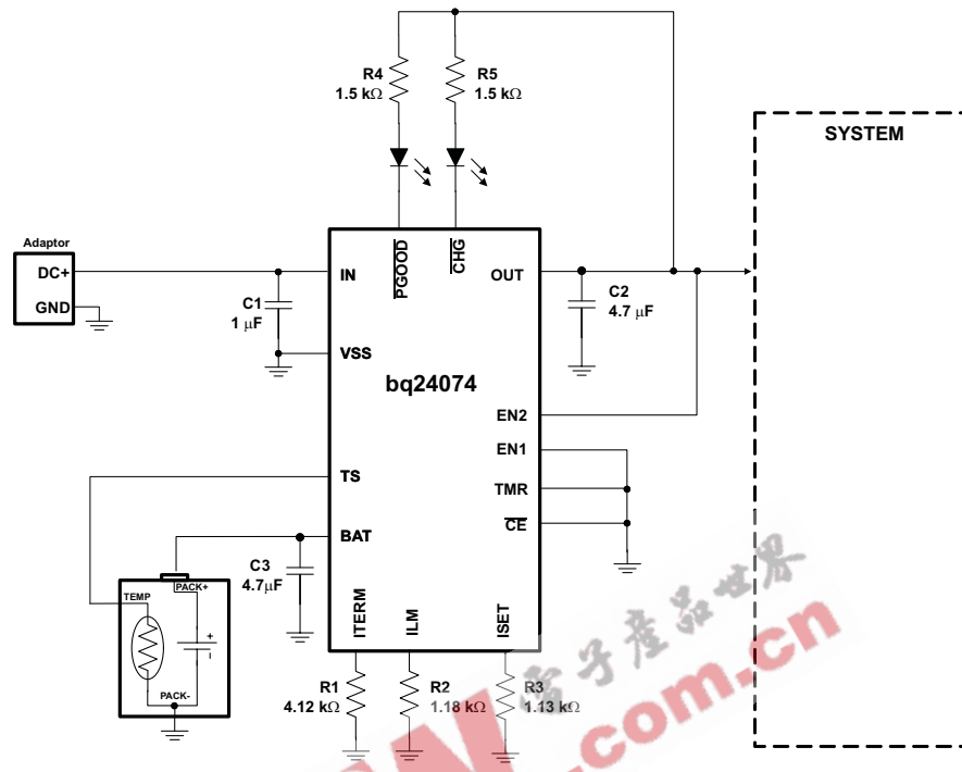
Figure 27. Using bq24074 in a Stand Alone Charger Application
