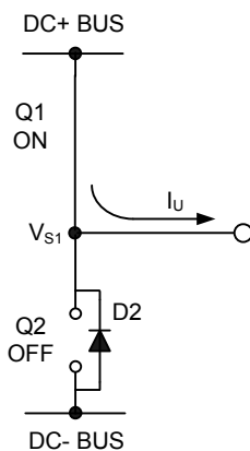
Figure 11: Q1 conducting
