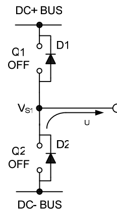
Figure 12: D2 conducting
