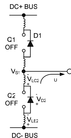
Figure 17: V_S negative
