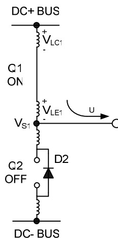
Figure 16: V_S positive
