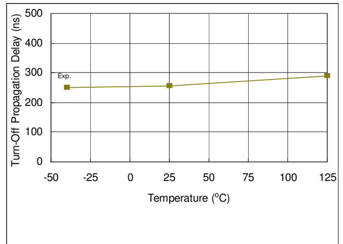
Fig. 23. Turn-off Propagation Delay vs. Temperature
