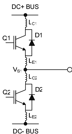
Figure 15: Parasitic Elements
