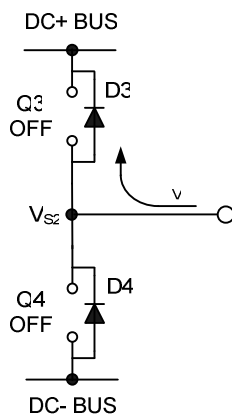
Figure 13: D3 conducting
